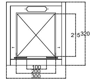
DETAIL LIFT SCALE BAR 1:10
