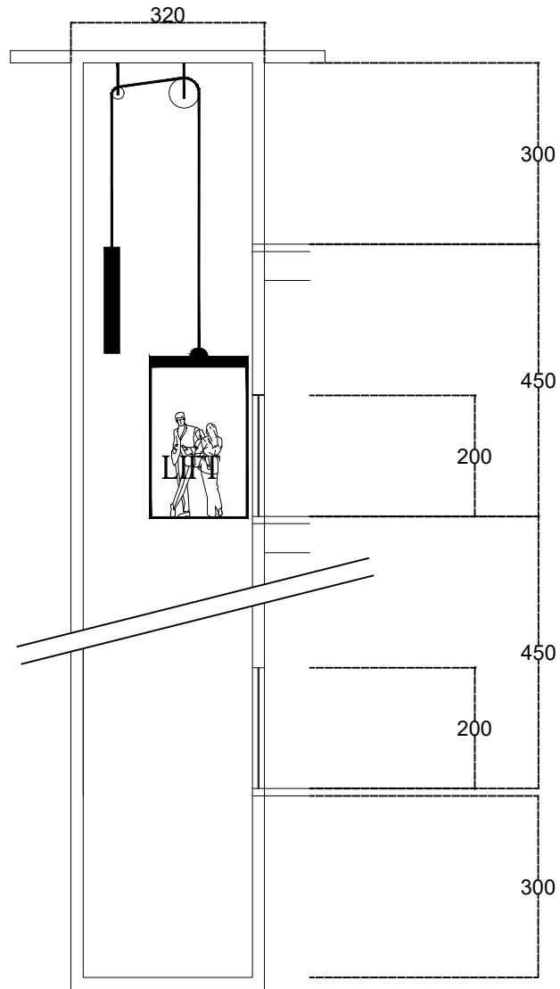
POTONGAN LIFT SCALE BAR 1:10
