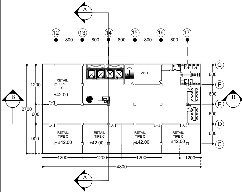
DENAH OFFICE LT 6-8
