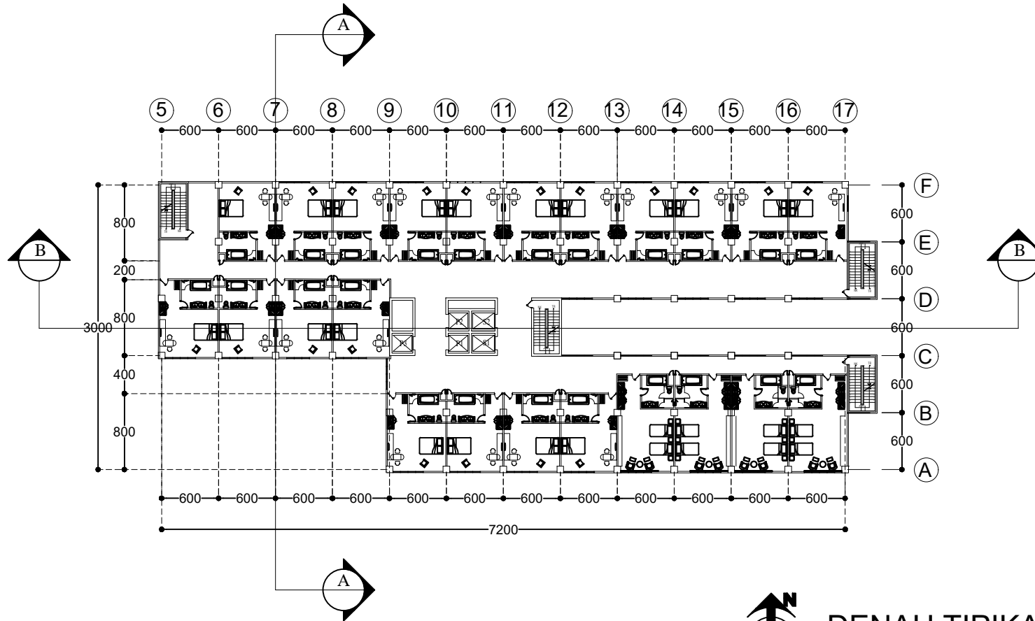
DENAH TIPIKAL LT 3-8
