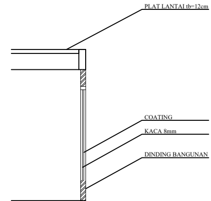
⊕ POTONGAN DETAIL FASAD SCALE BAR 1:10
