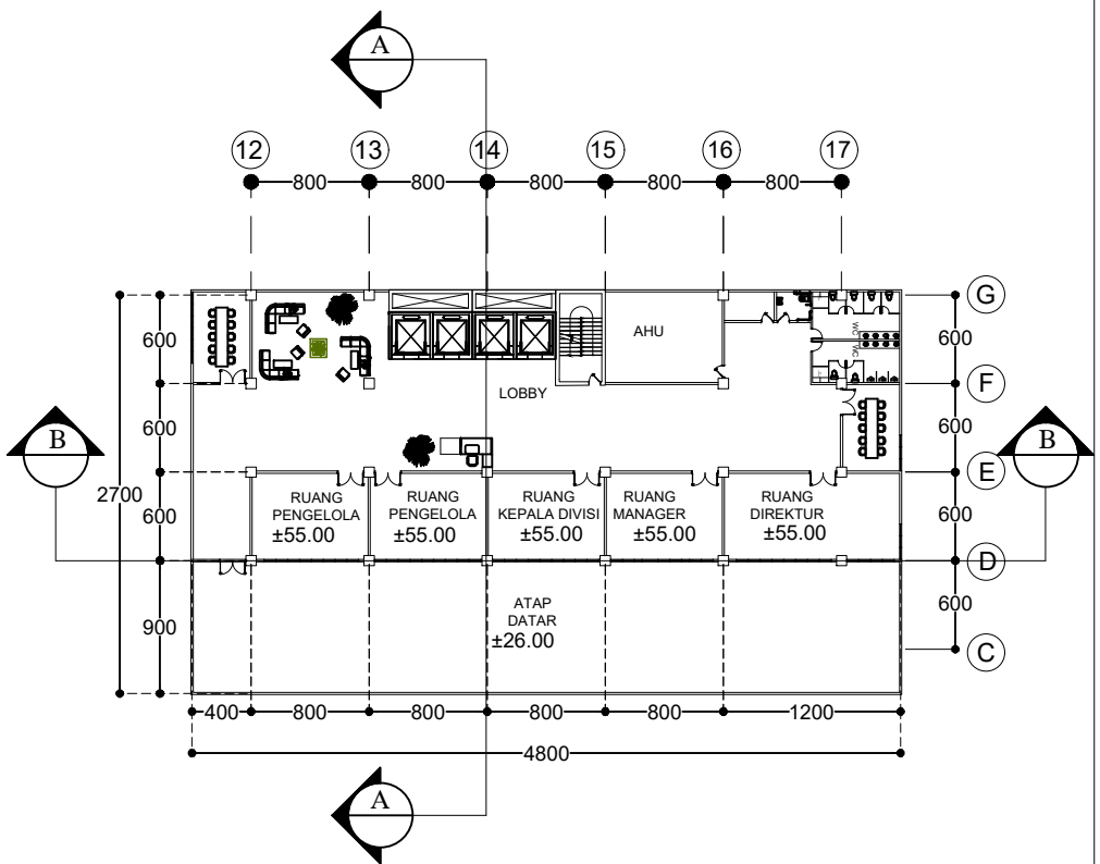
DENAH OFFICE LT 9
